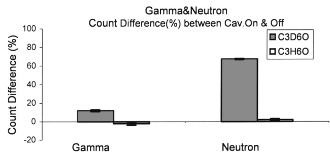
FIG. 9. Changes in gamma ray and neutron counts for tests with C_3D_6O and C_3H_6O at \sim 0^\circ C with and without cavitation. (PNG drive frequency=200 Hz. Acoustic drive frequencies= \sim 19.3 kHz and \sim 20.3 kHz for C_3D_6O and C_3H_6O ; error bars are 1 SD.)
