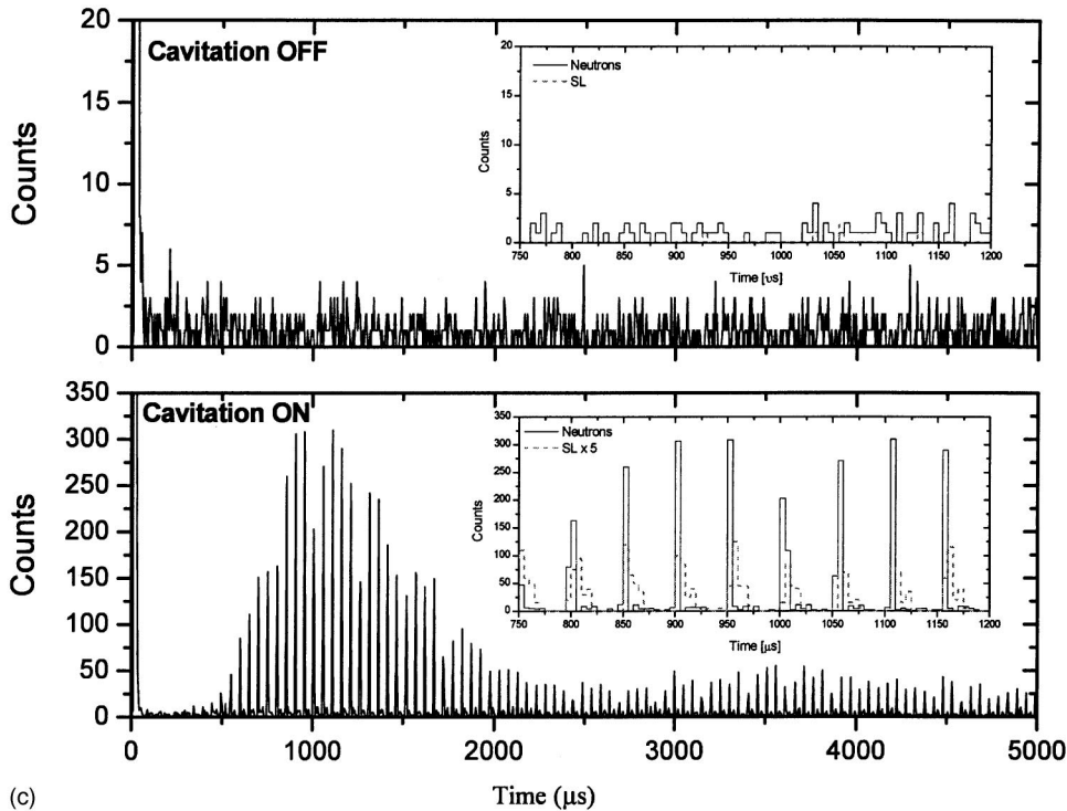
FIG. 7. (a) Change in neutron counts for chilled acetone with cavitation for the first 100 \mu s (acetone at 0 ^{\circ} C; PNG drive frequency \sim 200 Hz; acoustic forcing frequency = \sim 19.3 kHz; error bars are 1 SD). (b) Corresponding change in SL counts for acetone for first 100 \mu s. (c) Composite plots showing time correlation between neutron and SL counts over 5000 \mu s for cases of cavitation off and cavitation on (C 3 D 6 O at \sim 0 ^{\circ} C; PNG operation at 200 Hz). (d) Time correlation between neutron and SL counts between 0.5 and 2.0 msec. (Cavitation on–cavitation off; C 3 D 6 O at \sim 0 ^{\circ} C; PNG operation at \sim 200 Hz.) (e) Variation of aggregate neutron and SL counts in peak and in-between peak regions between 0.5 and 2.0 msec. (Cavitation on–cavitation off; C 3 D 6 O at \sim 0 ^{\circ} C; PNG operation at \sim 200 Hz. Neutron counts per channel in peak channels are about 50 times larger than for remaining channels; the corresponding SL counts per channel in peak channels are about 5 times larger.)
